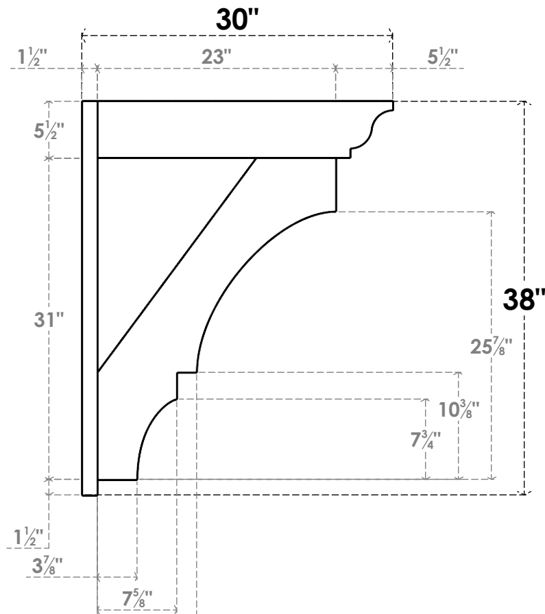
SIDE PROFILE
